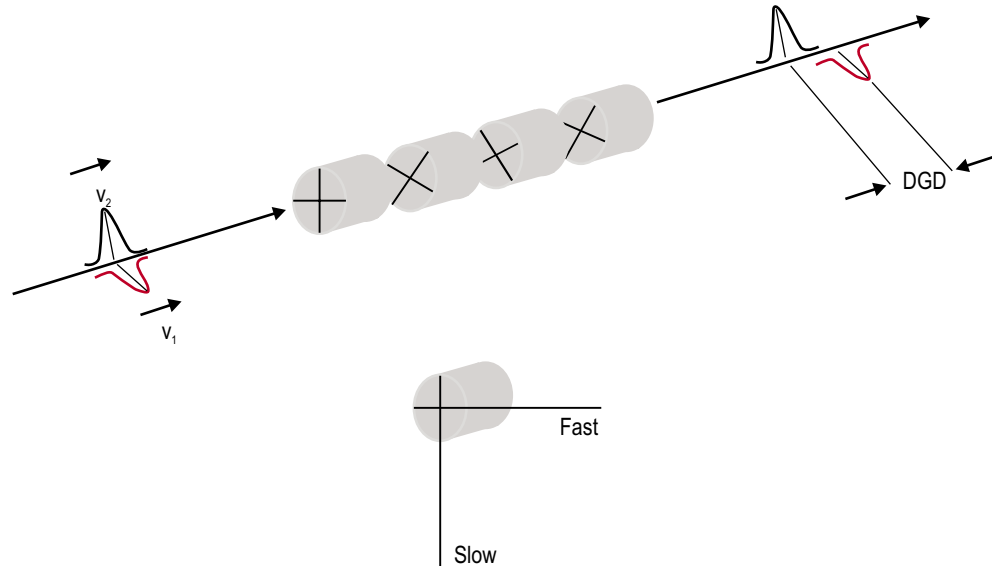
Figure 3: Strong mode coupling in telecommunication fibers
