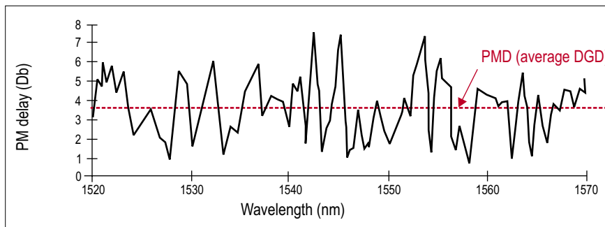
Figure 4: DGD variation over a wavelength range
