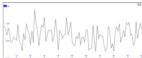
Figure 7: Drift representation of a long-term PMD delay measurement
