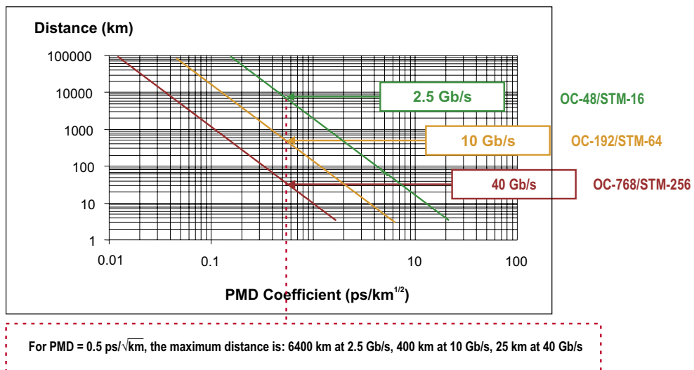
Figure 6: Maximum distance vs. PMD coefficient and data bit rate
