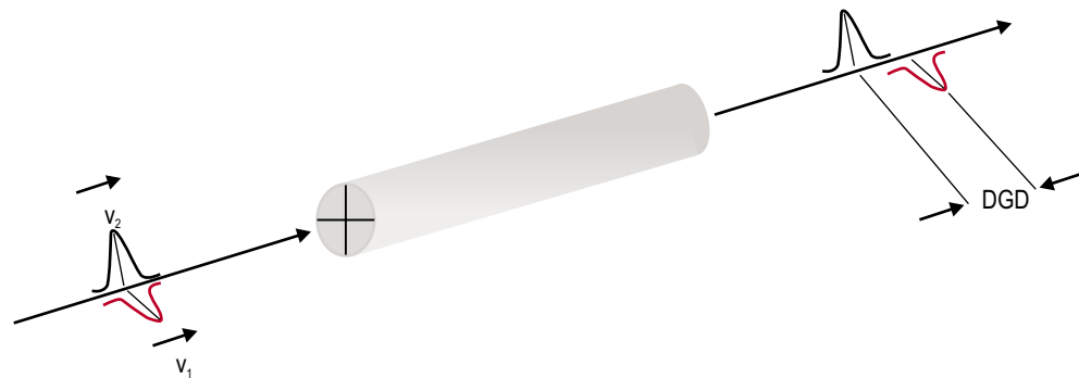
Figure 2: Differential group delay in HiBi fiber
