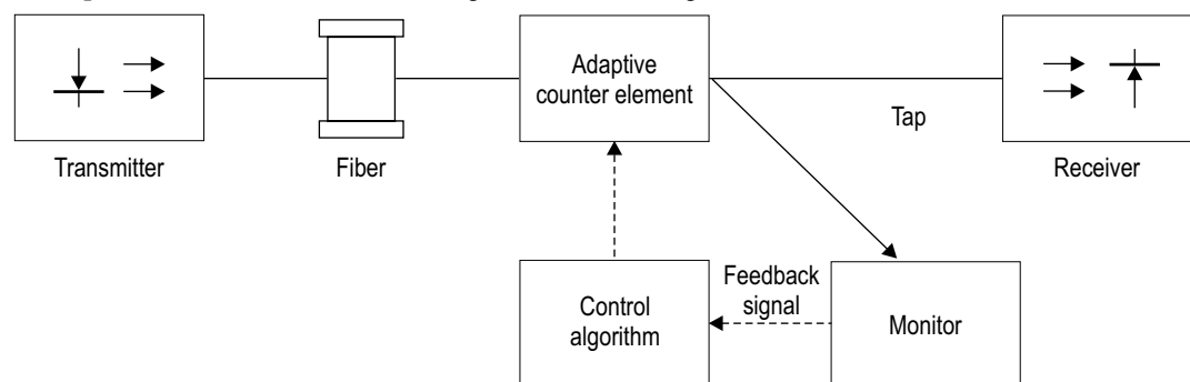
Figure 8: General scheme for optical PMD compensation
